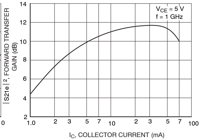
Figure 8. |S_{21e}|^2 - I_C
