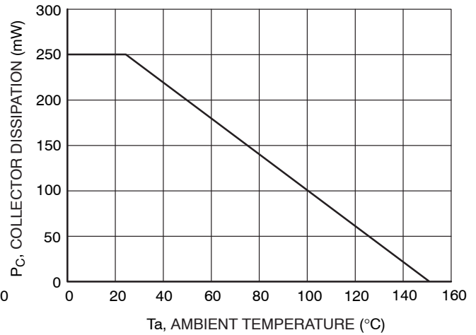
Figure 10. P_C - T_a
