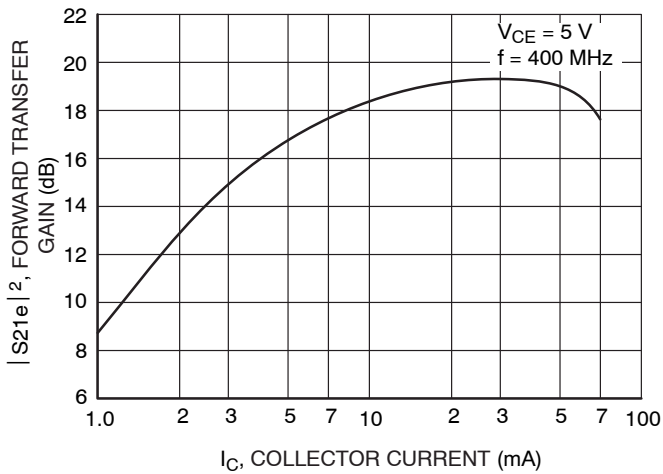
Figure 9. |S_{21e}|^2 - I_C
