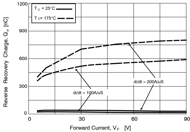
Figure 19. Stored Charge
