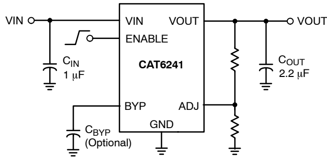
Figure 1. Application Schematic
