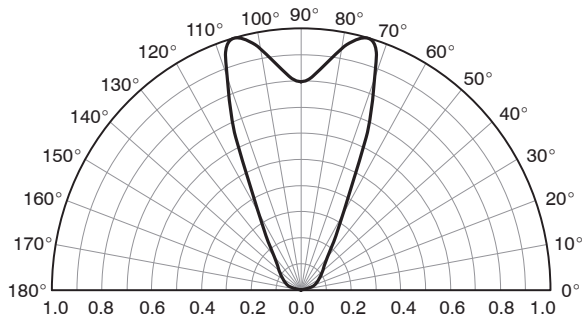
Figure 7. Radiation Diagram
